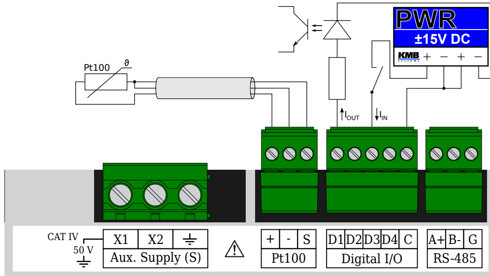
Figure 9: Connection of inputs and outputs in the device ARTIQ 233.
